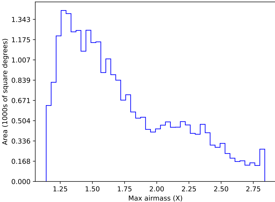
too_10_1v3.4_10yrs Yr 1 i band: Max airmass
