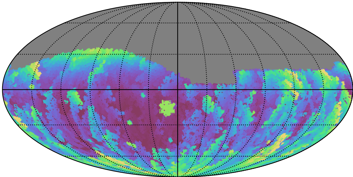
too_10_1v3.4_10yrs Yr 1 g band: Max airmass
