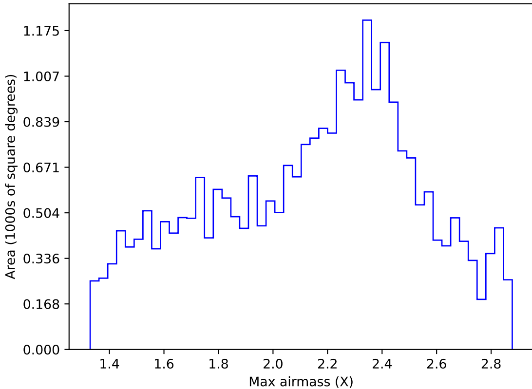
too_10_1v3.4_10yrs Yr 1 all bands: Max airmass
