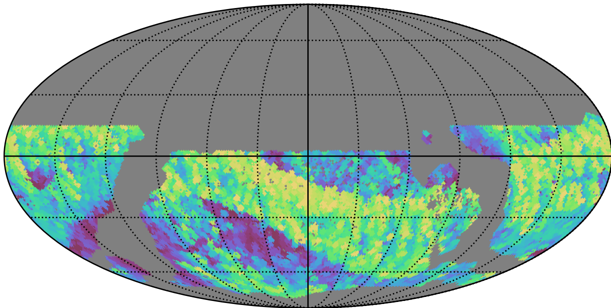
too_10_1v3.4_10yrs WFD z band: Max airmass
