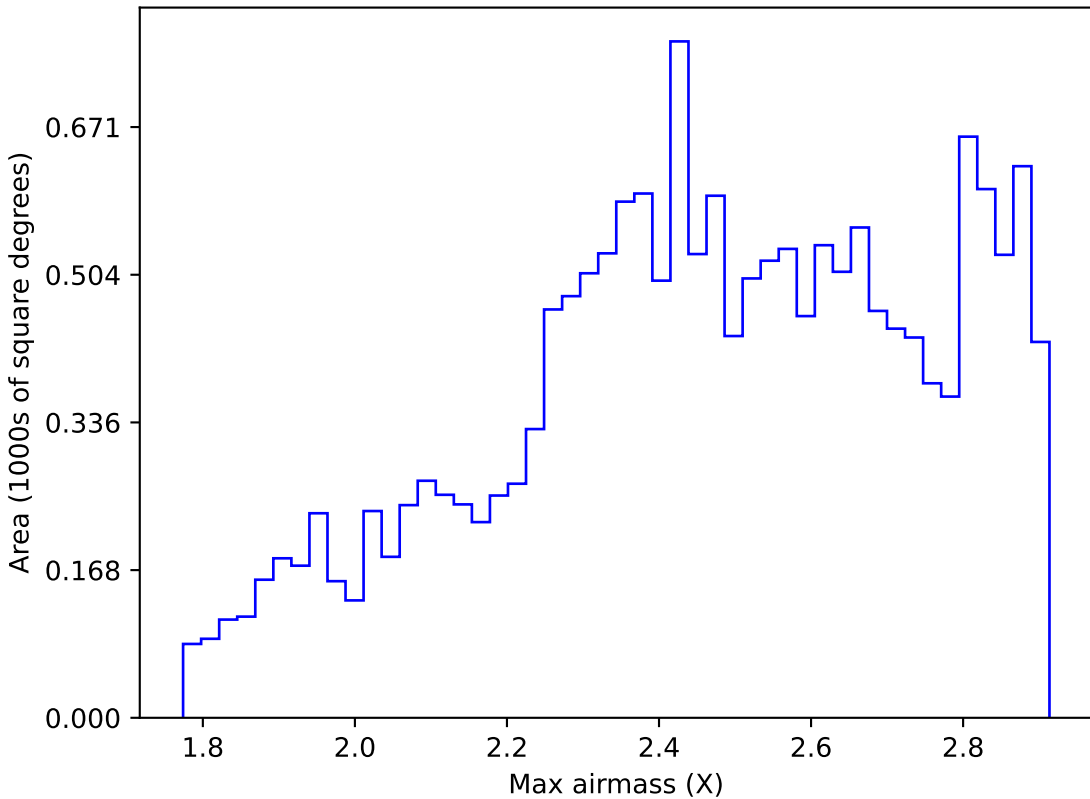
too_10_1v3.4_10yrs WFD z band: Max airmass
