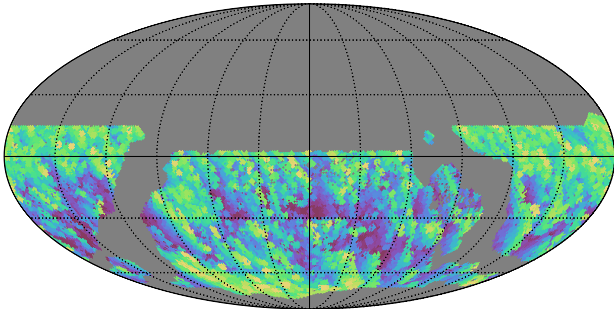
too_10_1v3.4_10yrs WFD y band: Max airmass
