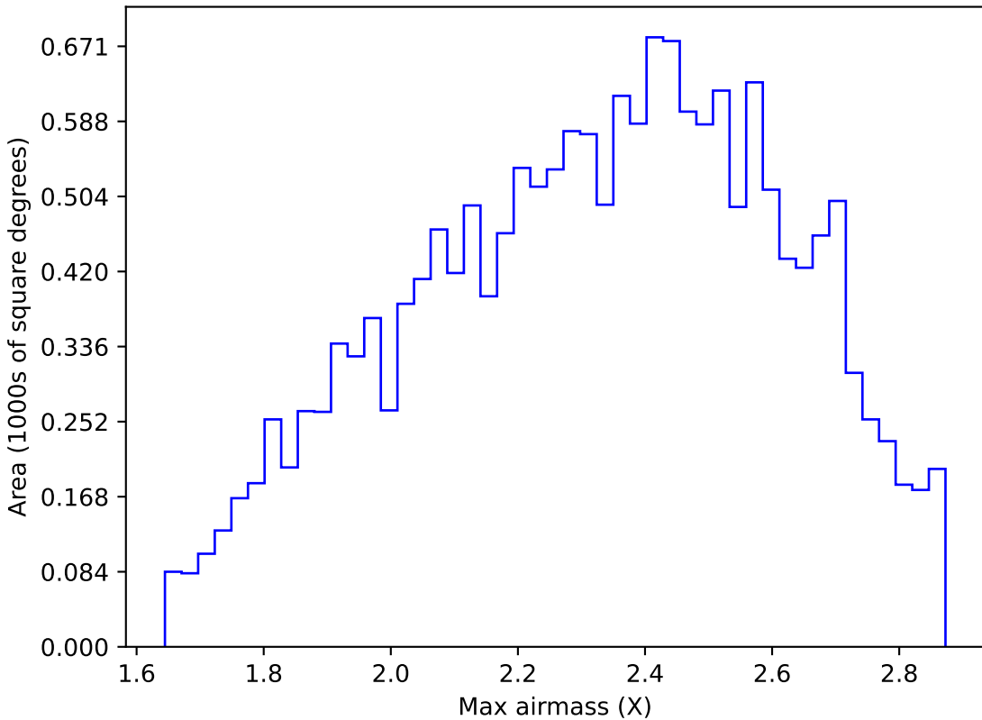
too_10_1v3.4_10yrs WFD y band: Max airmass
