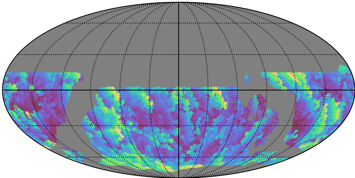
too_10_1v3.4_10yrs WFD u band: Max airmass
