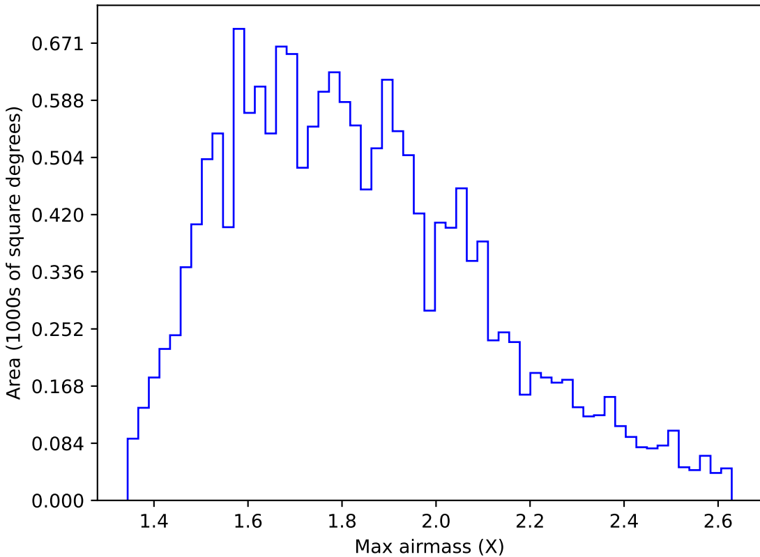
too_10_1v3.4_10yrs WFD u band: Max airmass
