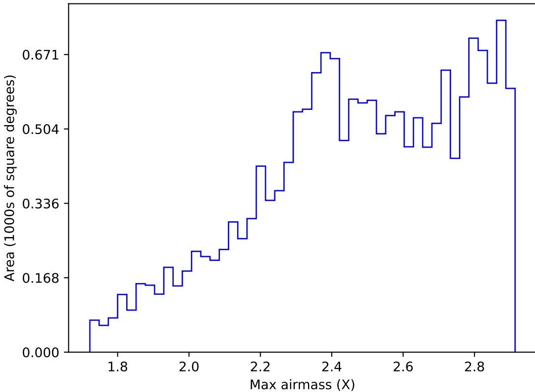
too_10_1v3.4_10yrs WFD i band: Max airmass
