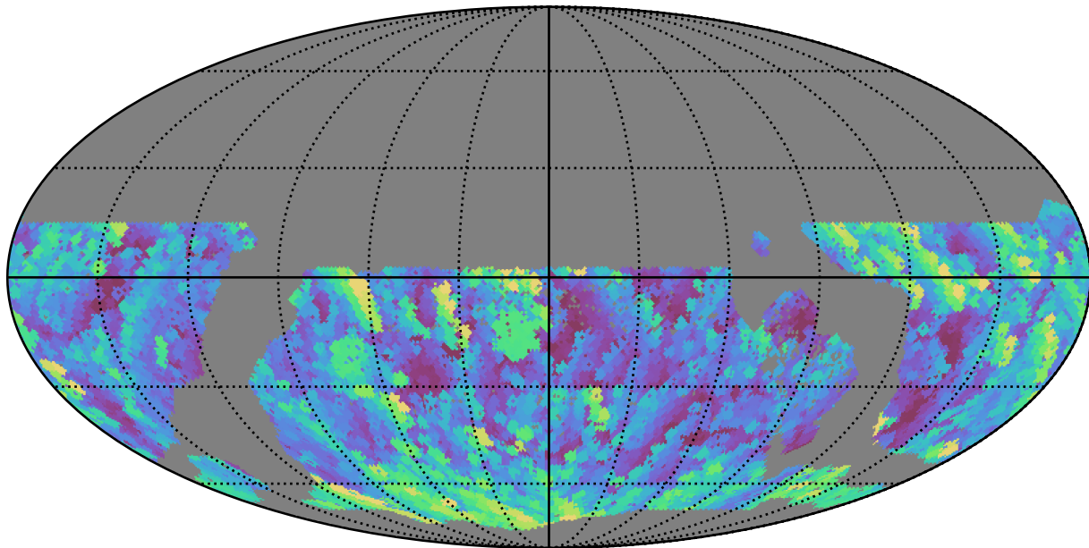
too_10_1v3.4_10yrs WFD g band: Max airmass
