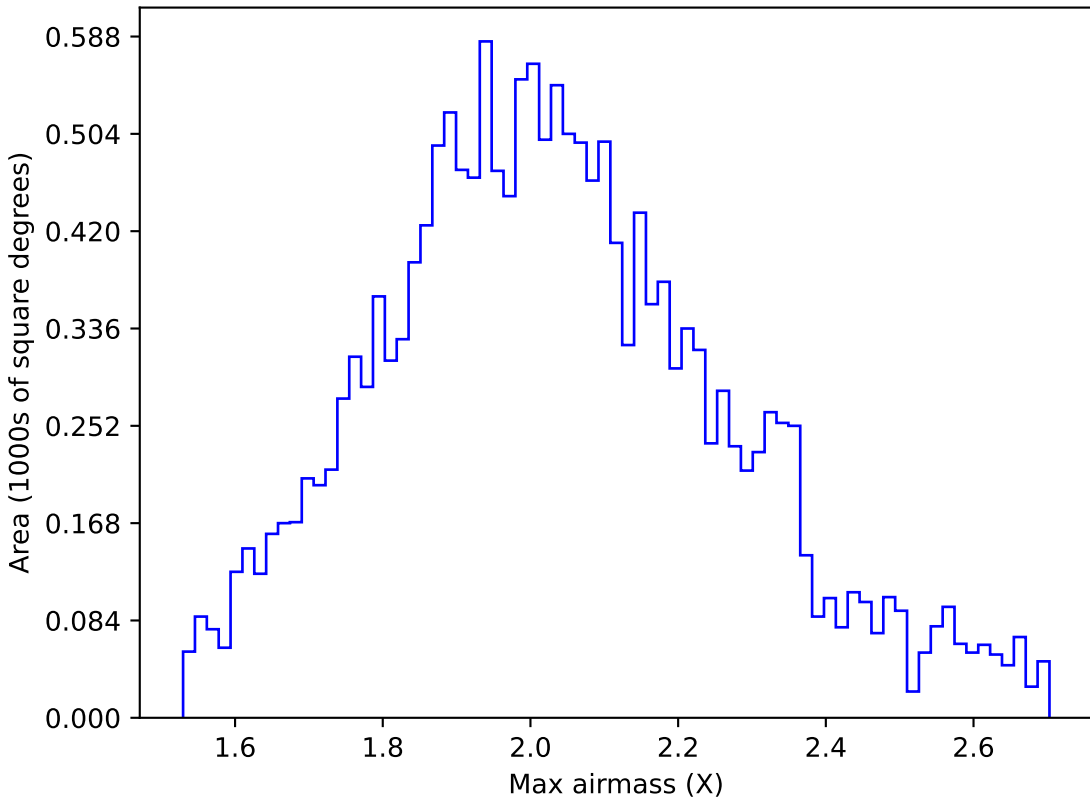
too_10_1v3.4_10yrs WFD g band: Max airmass
