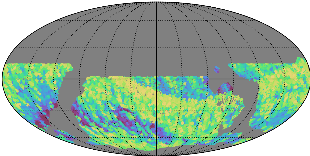
too_10_1v3.4_10yrs WFD all bands: Max airmass
