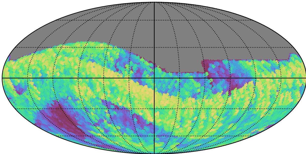
too_10_1v3.4_10yrs All sky z band: Max airmass
