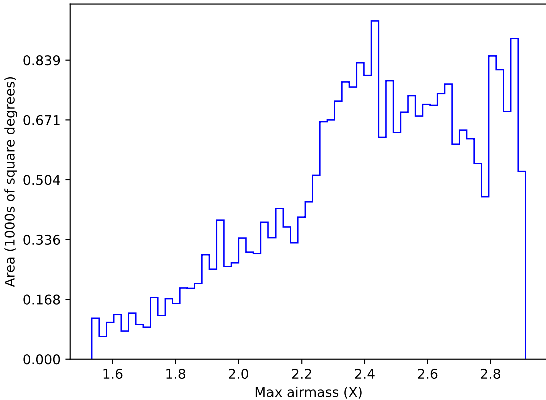
too_10_1v3.4_10yrs All sky z band: Max airmass
