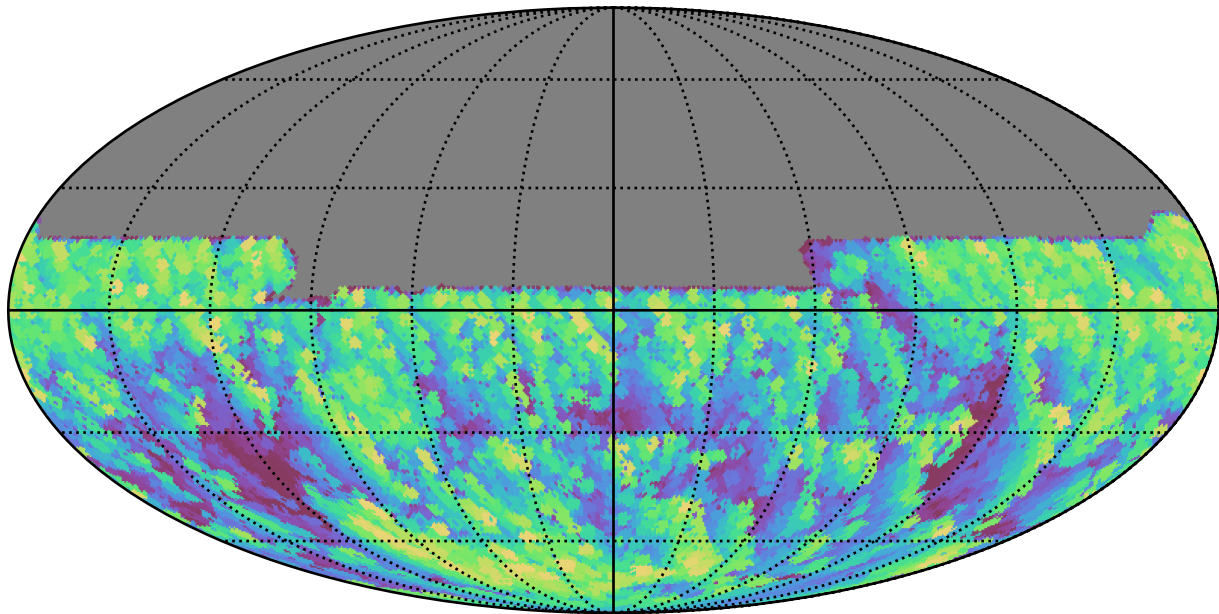
too_10_1v3.4_10yrs All sky y band: Max airmass
