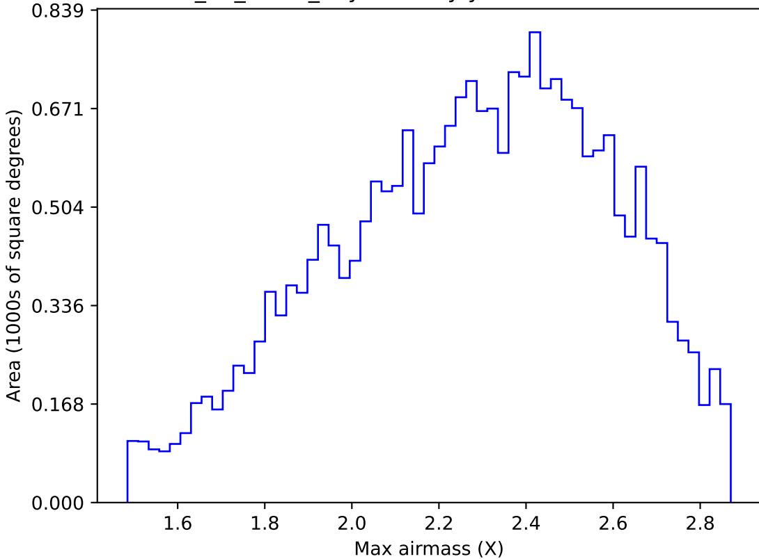
too_10_1v3.4_10yrs All sky y band: Max airmass
