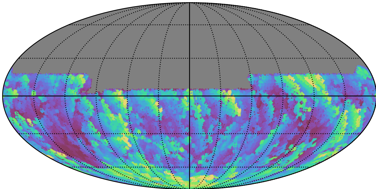
too_10_1v3.4_10yrs All sky u band: Max airmass
