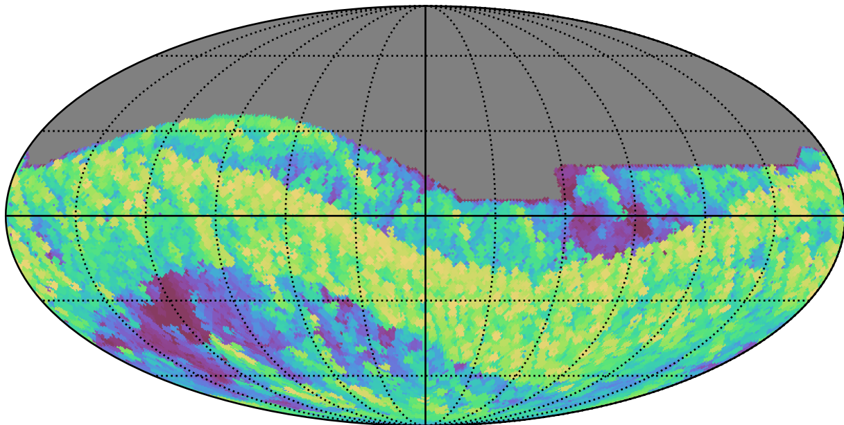
too_10_1v3.4_10yrs All sky i band: Max airmass
