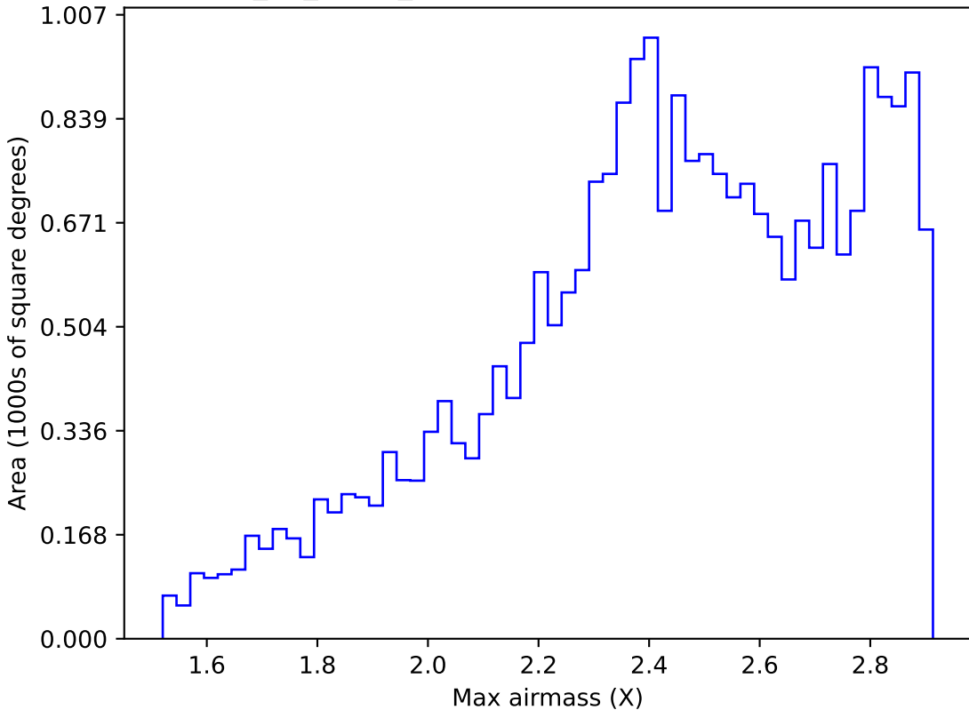
too_10_1v3.4_10yrs All sky i band: Max airmass
