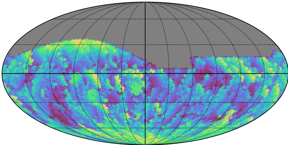
too_10_1v3.4_10yrs All sky g band: Max airmass
