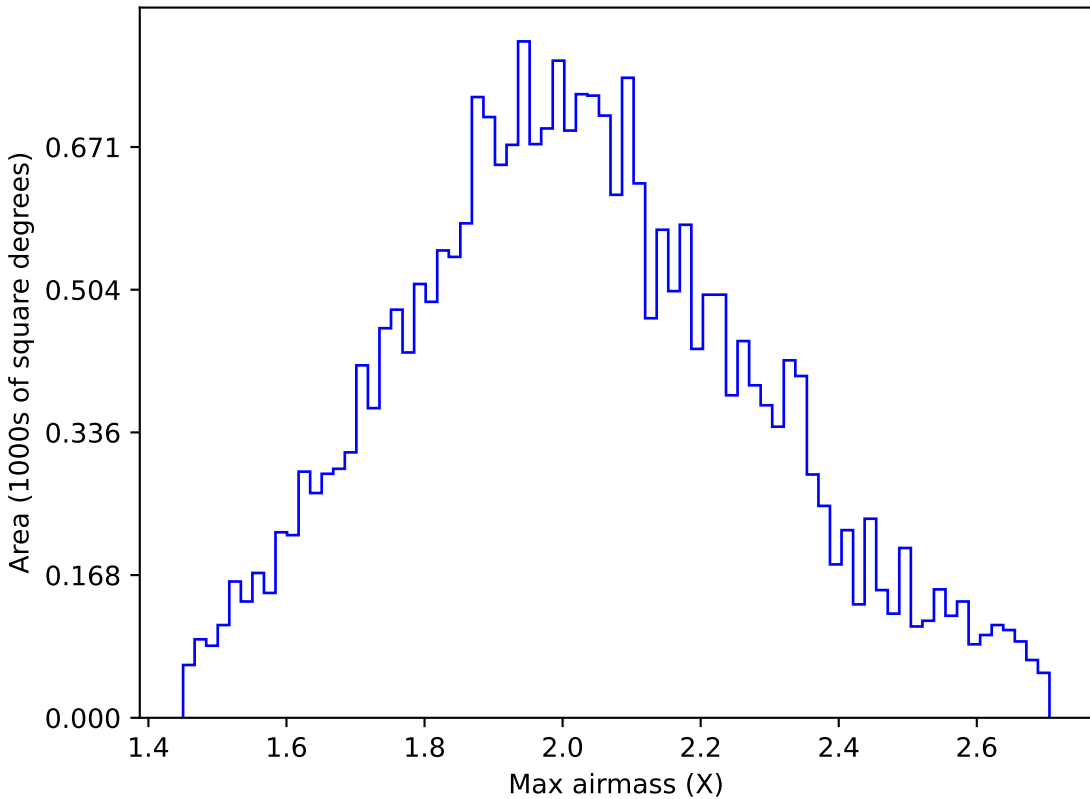
too_10_1v3.4_10yrs All sky g band: Max airmass
