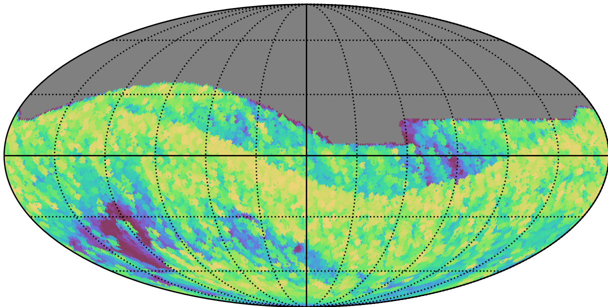
too_10_1v3.4_10yrs All sky all bands: Max airmass
