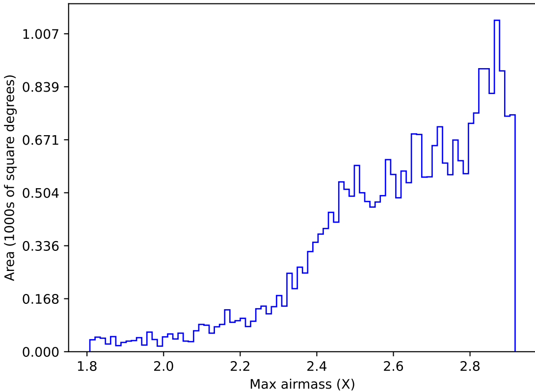
too_10_1v3.4_10yrs All sky all bands: Max airmass
