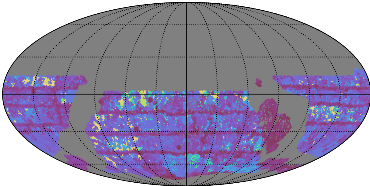
too_10_1v3.4_10yrs WFD z band: Max Inter-Night Gap
