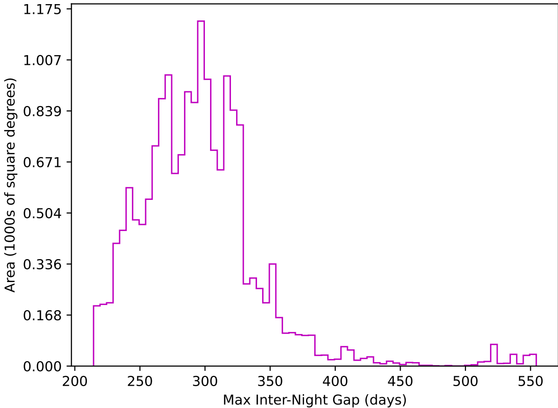
too_10_1v3.4_10yrs WFD z band: Max Inter-Night Gap
