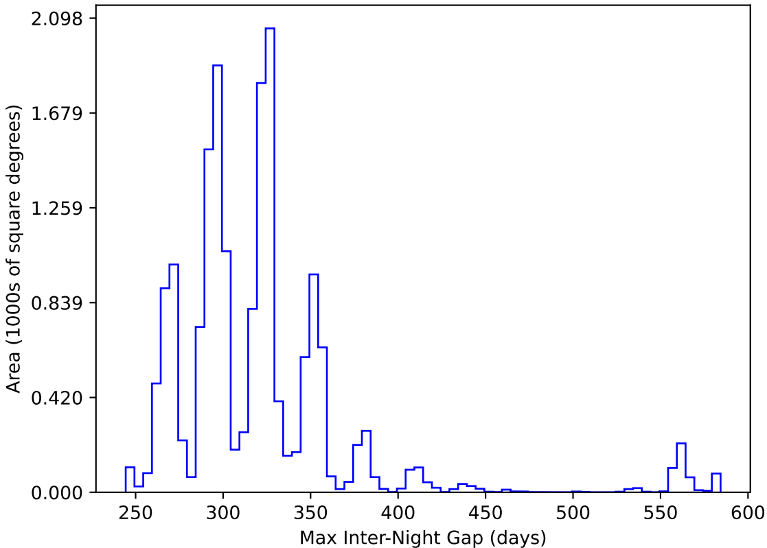
too_10_1v3.4_10yrs WFD y band: Max Inter-Night Gap
