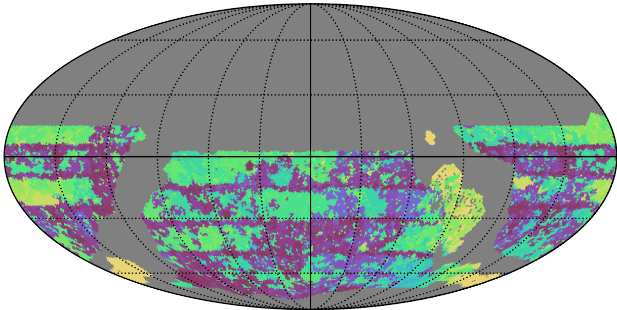
too_10_1v3.4_10yrs WFD u band: Max Inter-Night Gap
