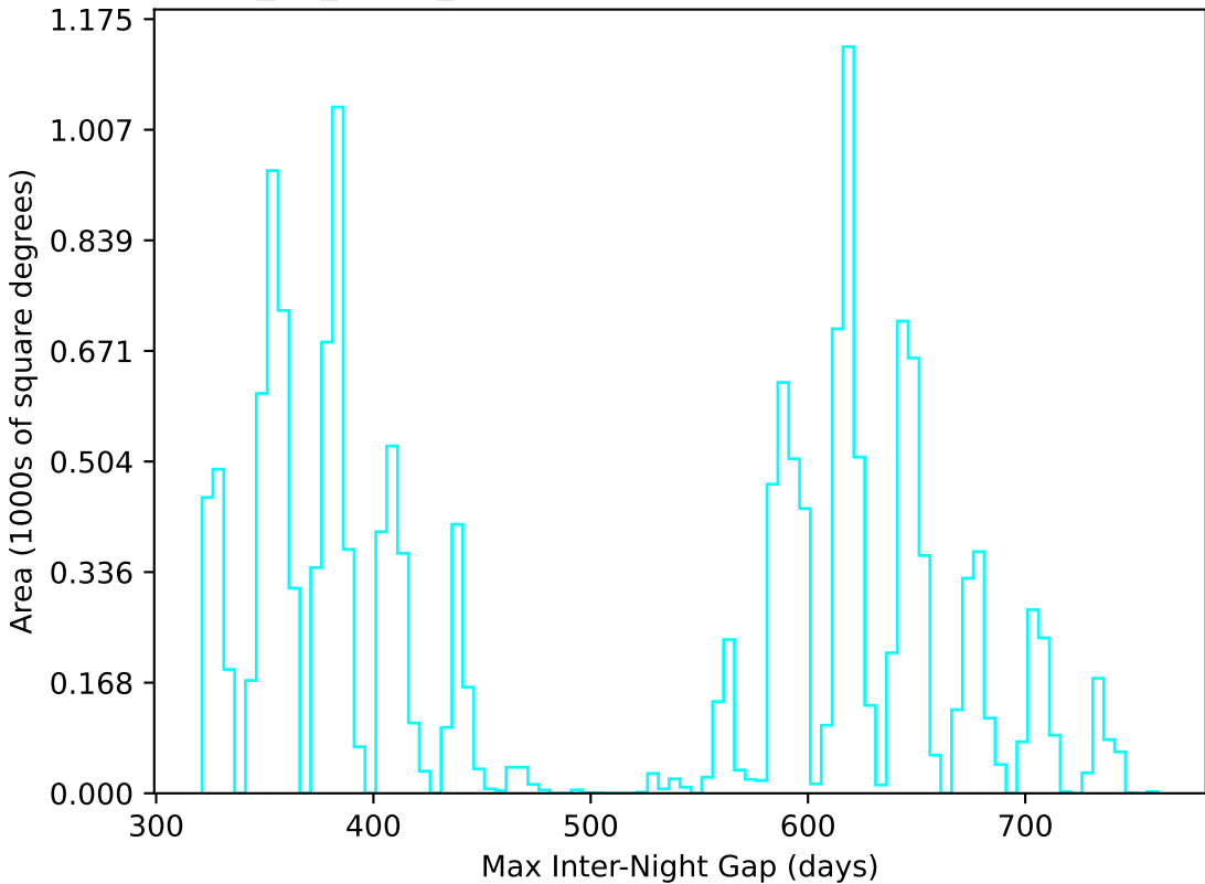
too_10_1v3.4_10yrs WFD u band: Max Inter-Night Gap
