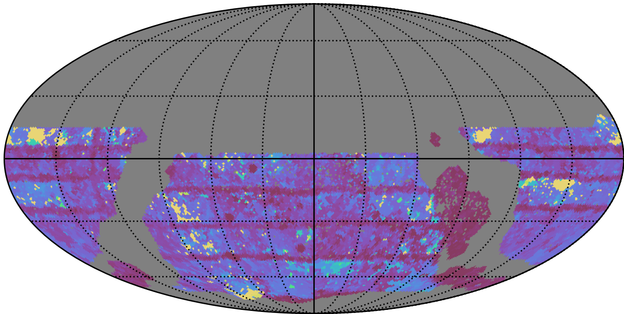
too_10_1v3.4_10yrs WFD i band: Max Inter-Night Gap
