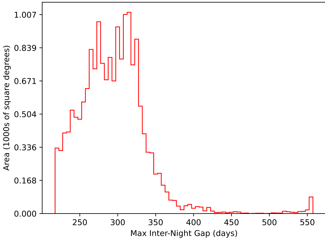
too_10_1v3.4_10yrs WFD i band: Max Inter-Night Gap
