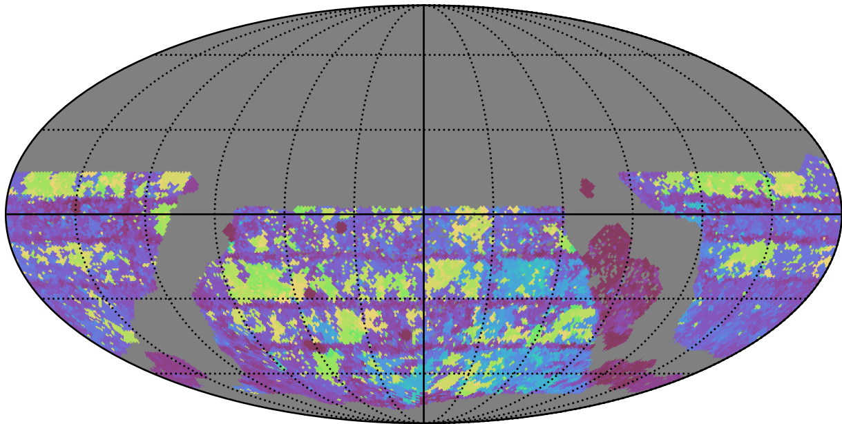
too_10_1v3.4_10yrs WFD g band: Max Inter-Night Gap
