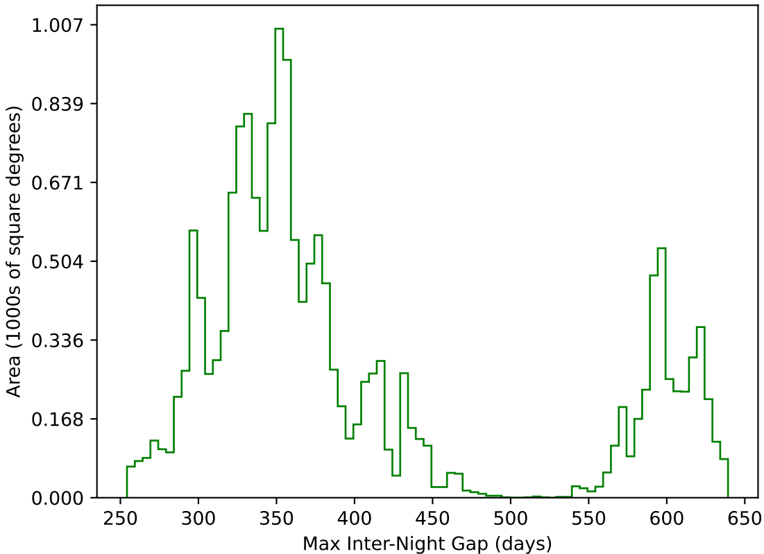
too_10_1v3.4_10yrs WFD g band: Max Inter-Night Gap
