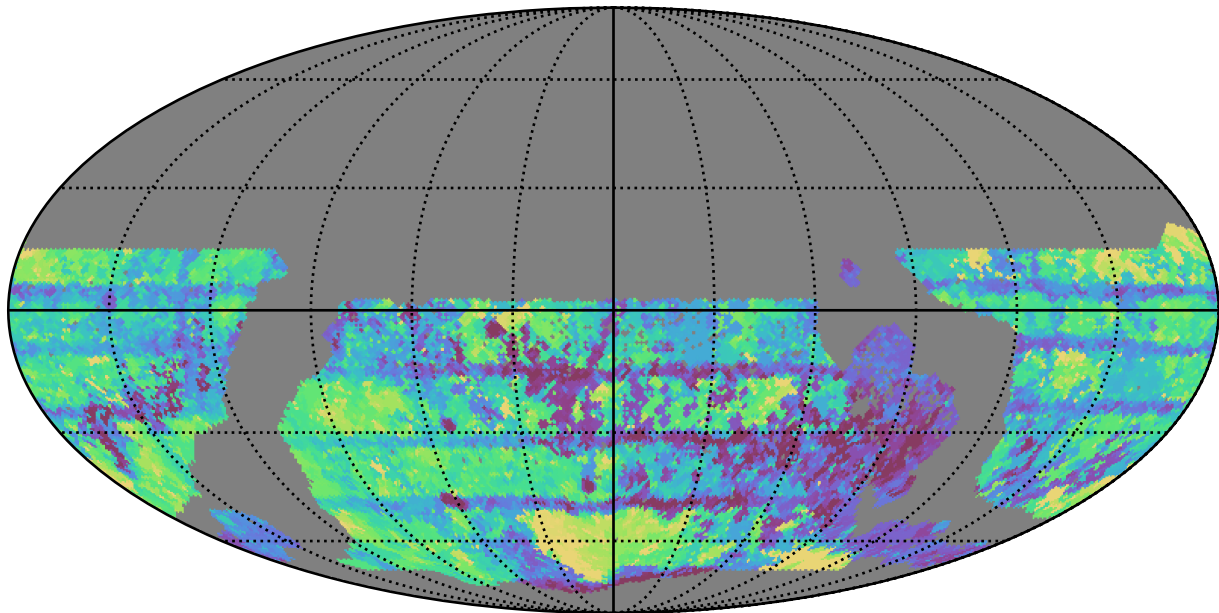
too_10_1v3.4_10yrs WFD all bands: Max Inter-Night Gap
