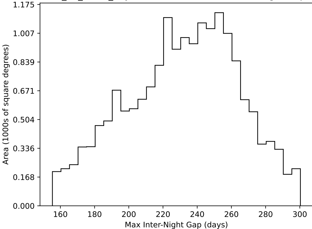
too_10_1v3.4_10yrs WFD all bands: Max Inter-Night Gap
