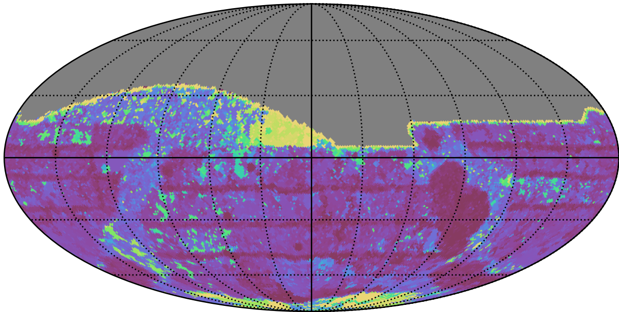
too_10_1v3.4_10yrs All sky z band: Max Inter-Night Gap
