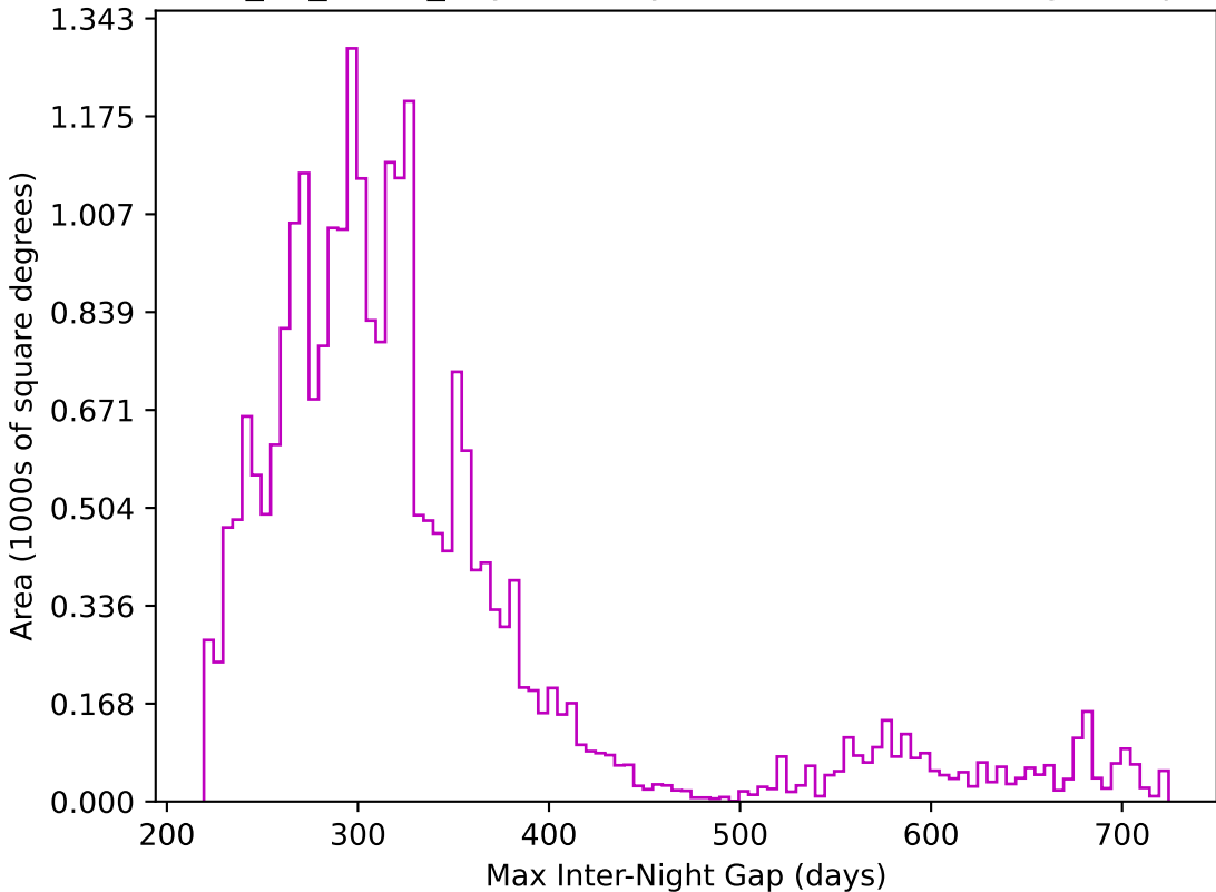
too_10_1v3.4_10yrs All sky z band: Max Inter-Night Gap
