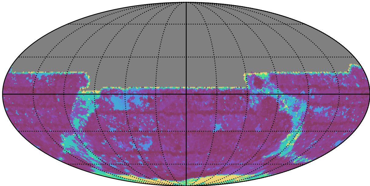
too_10_1v3.4_10yrs All sky y band: Max Inter-Night Gap
