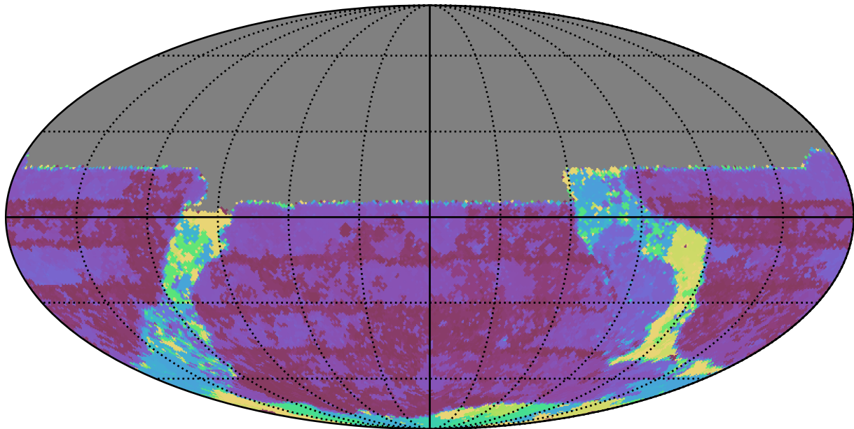
too_10_1v3.4_10yrs All sky u band: Max Inter-Night Gap
