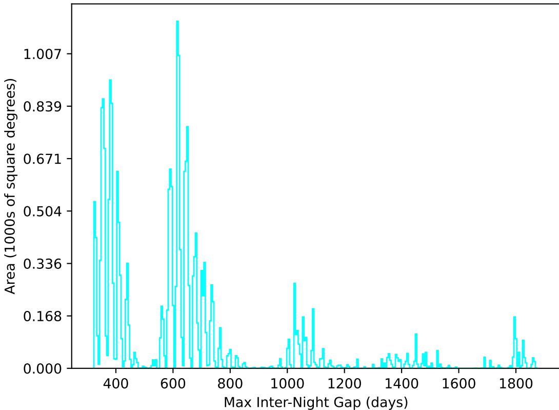
too_10_1v3.4_10yrs All sky u band: Max Inter-Night Gap
