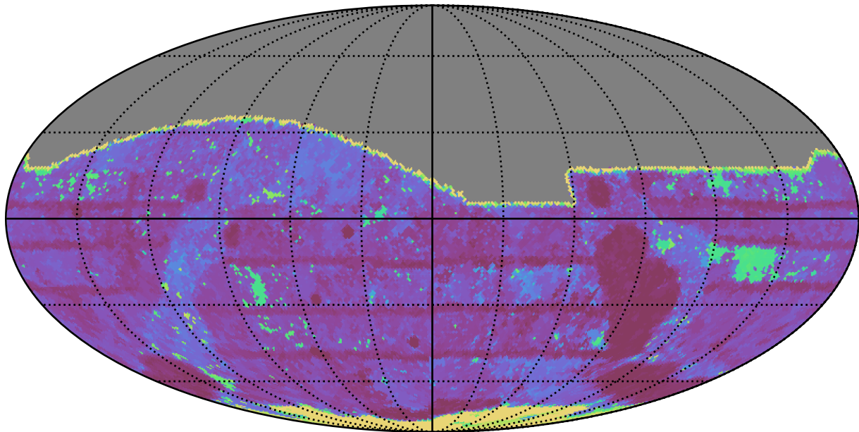
too_10_1v3.4_10yrs All sky r band: Max Inter-Night Gap
