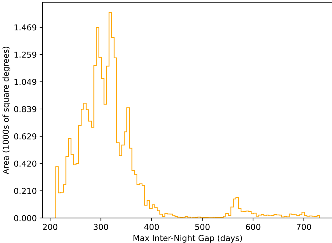
too_10_1v3.4_10yrs All sky r band: Max Inter-Night Gap
