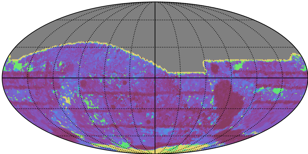
too_10_1v3.4_10yrs All sky i band: Max Inter-Night Gap
