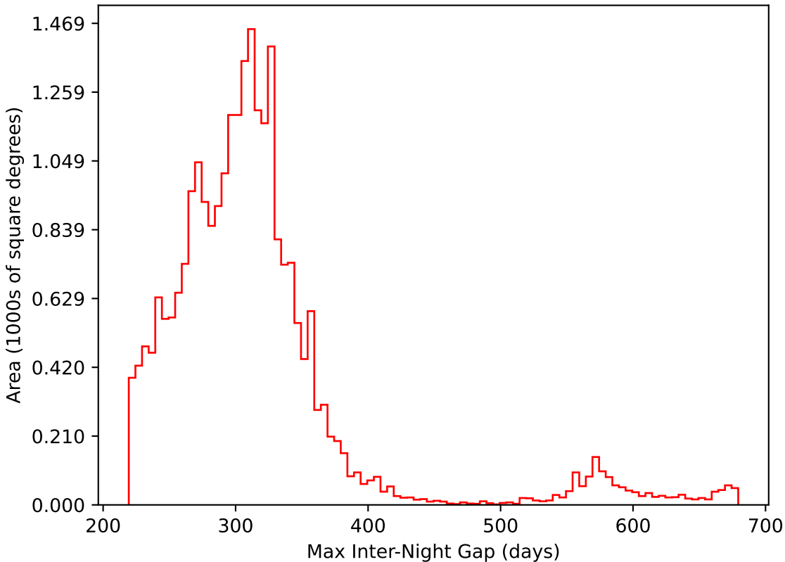
too_10_1v3.4_10yrs All sky i band: Max Inter-Night Gap
