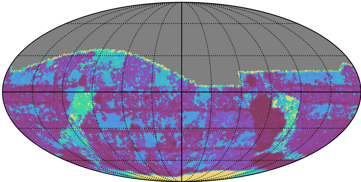
too_10_1v3.4_10yrs All sky g band: Max Inter-Night Gap
