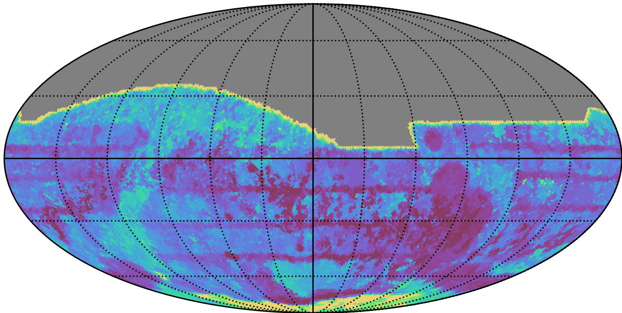
too_10_1v3.4_10yrs All sky all bands: Max Inter-Night Gap
