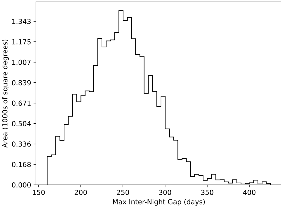
too_10_1v3.4_10yrs All sky all bands: Max Inter-Night Gap
