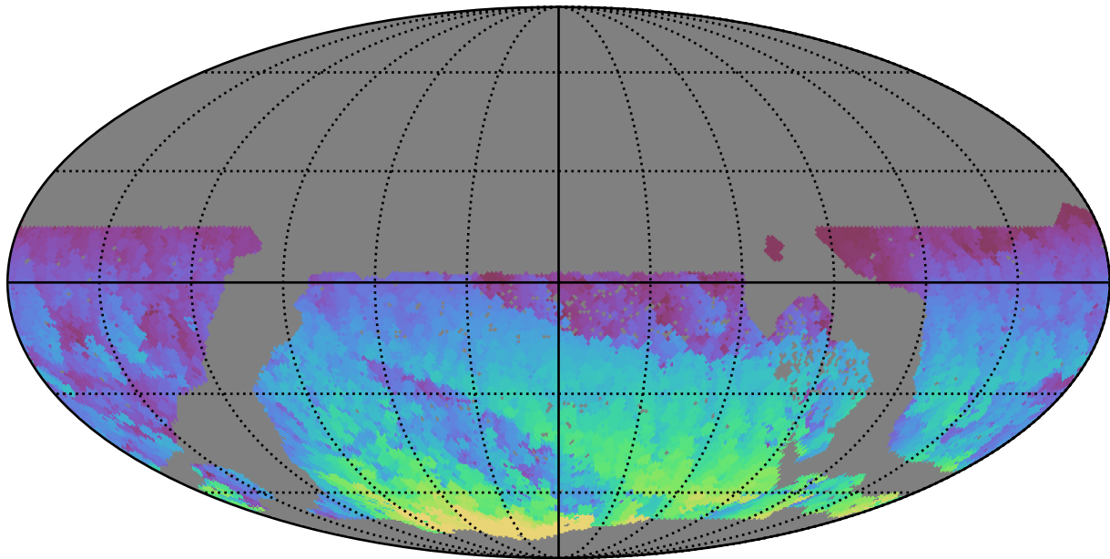
too_10_1v3.4_10yrs WFD z band: Max HA
