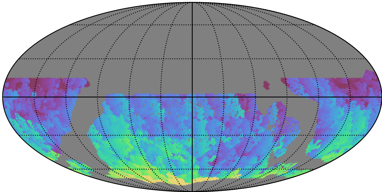
too_10_1v3.4_10yrs WFD u band: Max HA
