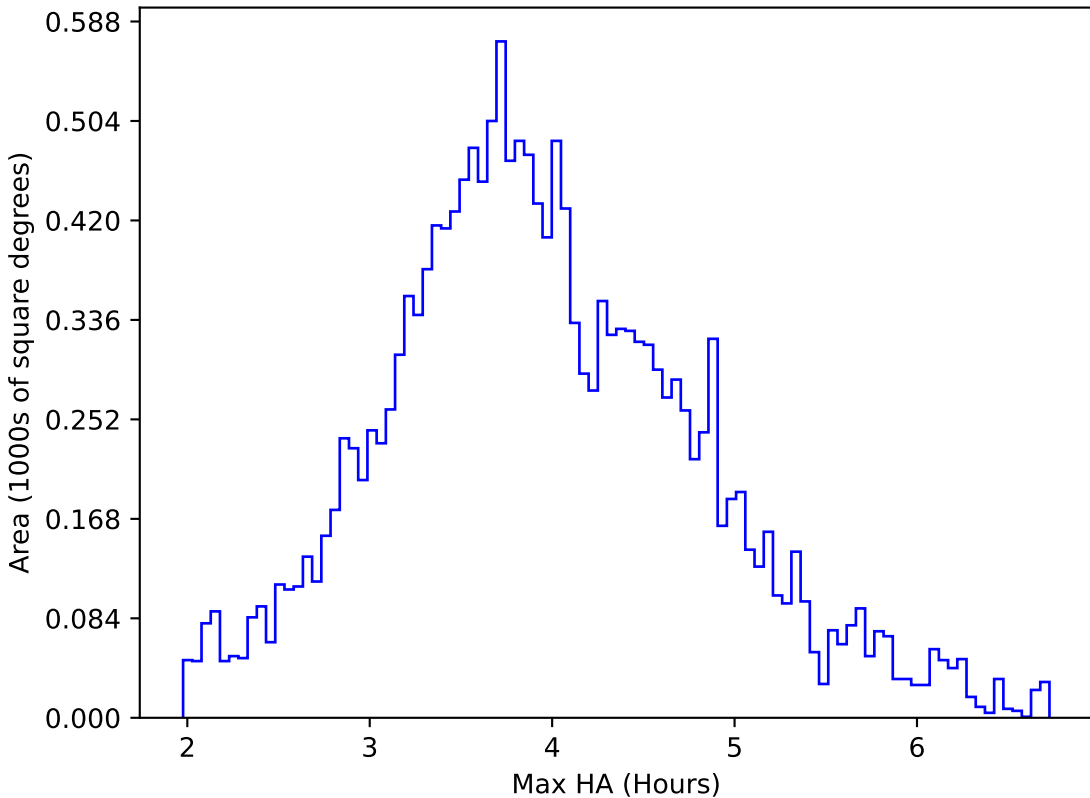
too_10_1v3.4_10yrs WFD u band: Max HA
